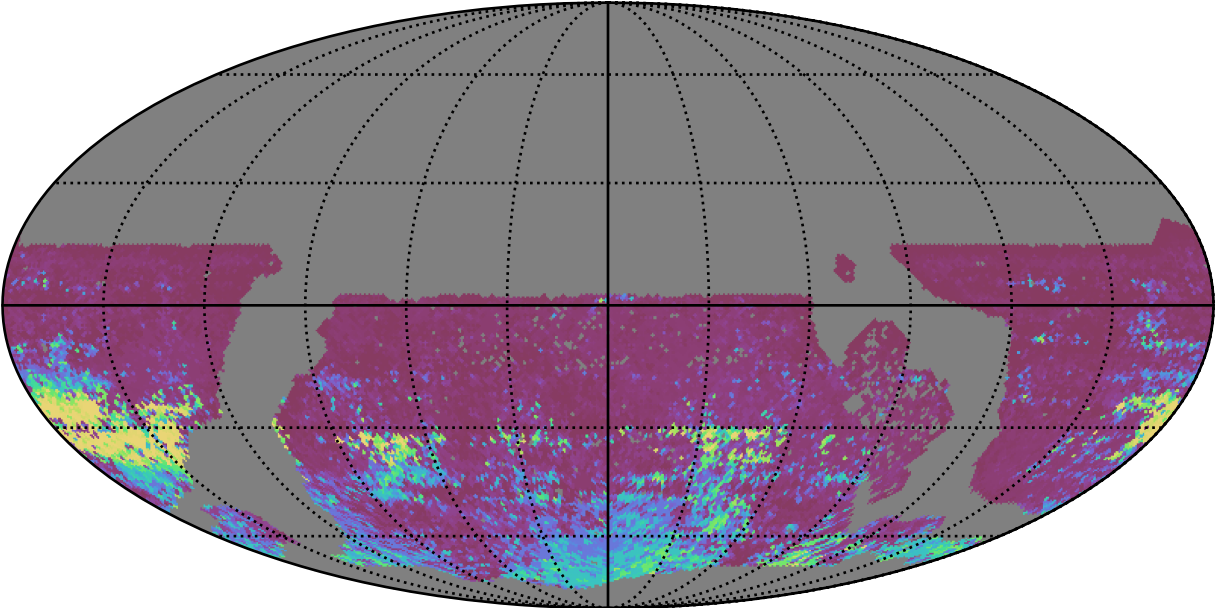
ddf_acor_sf20_lsf0_lsr0_v3.4_10yrs WFD r band: 75th Percentile Intranight Timespan
