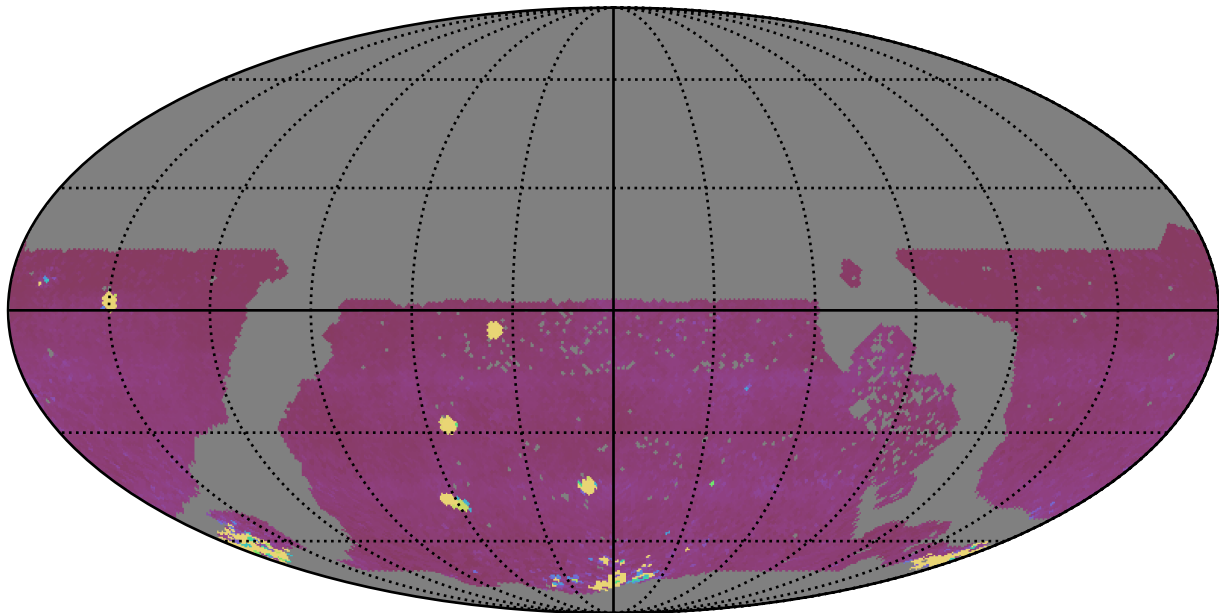
ddf_acor_sf20_lsf0_lsr0_v3.4_10yrs WFD iz bands: 75th Percentile Intranight Timespan
