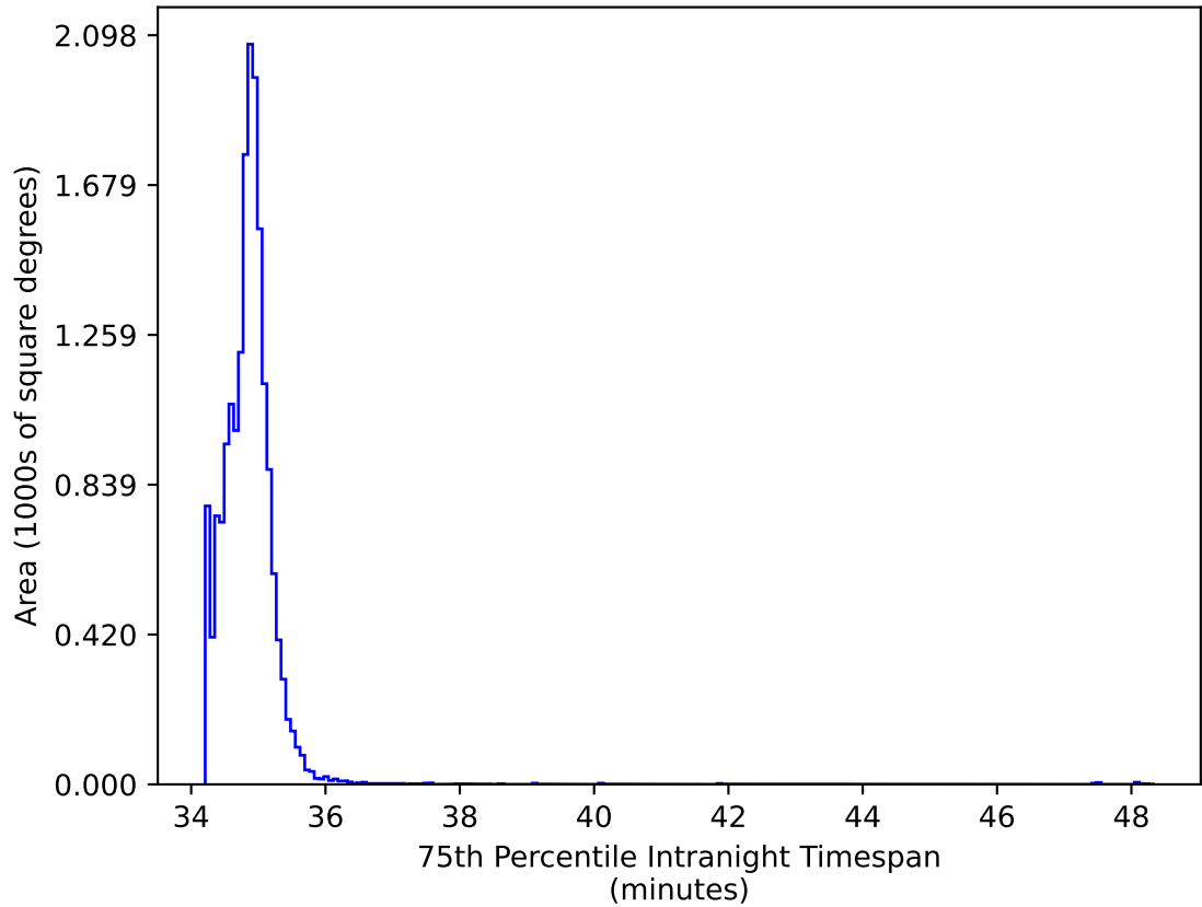
ddf_acor_sf20_lsf0_lsr0_v3.4_10yrs WFD iz bands: 75th Percentile Intranight Timespan
