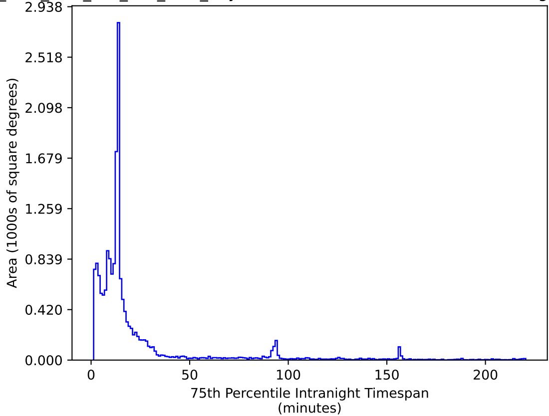
ddf_acor_sf20_lsf0_lsr0_v3.4_10yrs WFD i band: 75th Percentile Intranight Timespan
