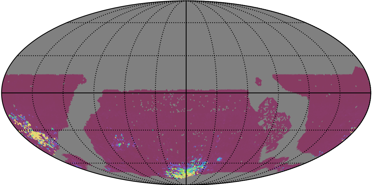
ddf_acor_sf20_lsf0_lsr0_v3.4_10yrs WFD gr bands: 75th Percentile Intranight Timespan
