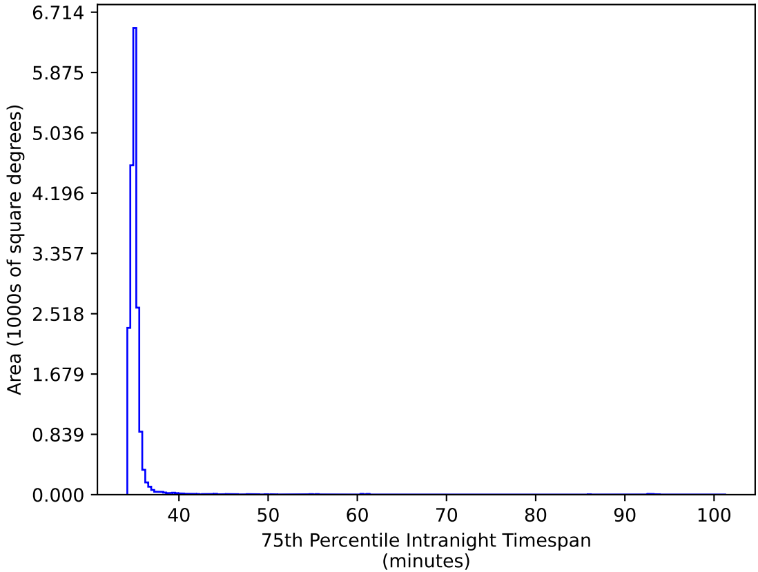
ddf_acor_sf20_lsf0_lsr0_v3.4_10yrs WFD gr bands: 75th Percentile Intranight Timespan
