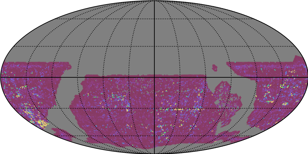
ddf_acor_sf20_lsf0_lsr0_v3.4_10yrs WFD g band: 75th Percentile Intranight Timespan
