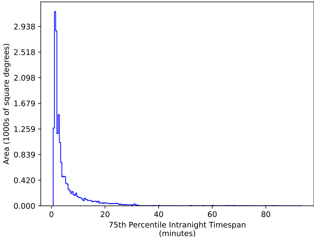
ddf_acor_sf20_lsf0_lsr0_v3.4_10yrs WFD g band: 75th Percentile Intranight Timespan
