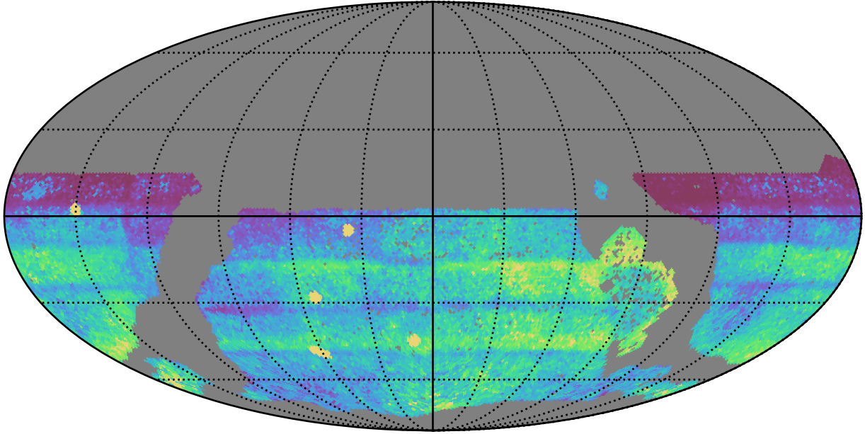
ddf_acor_sf20_lsr0_v3.4_10yrs WFD all bands: 75th Percentile Intranight Timespan
