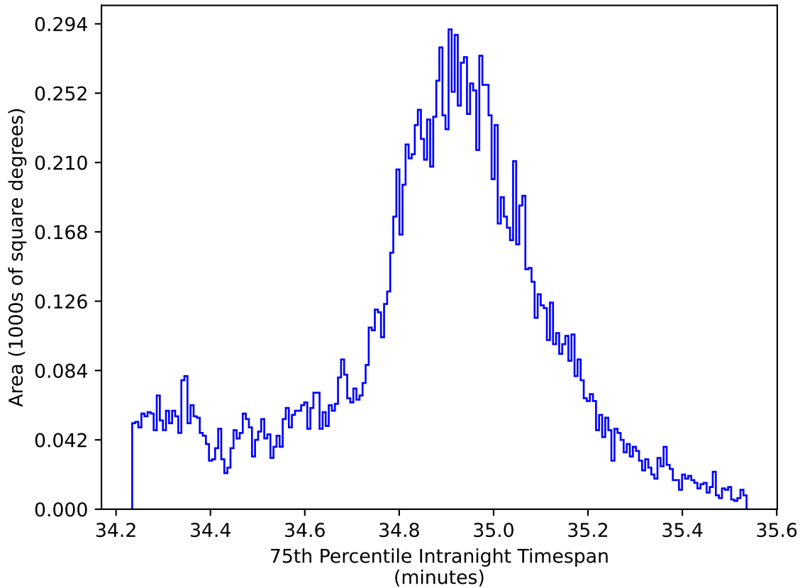
ddf_acor_sf20_lsf0_lsr0_v3.4_10yrs WFD all bands: 75th Percentile Intranight Timespan
