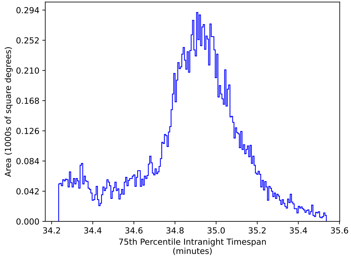
ddf_acor_sf20_lsf0_lsr0_v3.4_10yrs WFD: 75th Percentile Intranight Timespan
