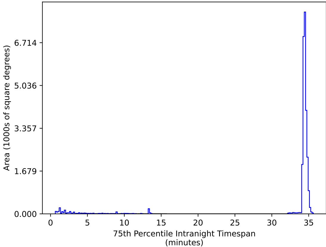
ddf_acor_sf20_lsf0_lsr0_v3.4_10yrs All sky zy bands: 75th Percentile Intranight Timespan
