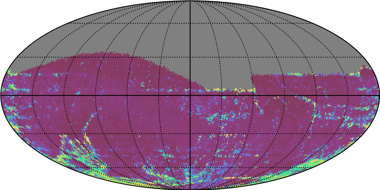
ddf_acor_sf20_lsf0_lsr0_v3.4_10yrs All sky z band: 75th Percentile Intranight Timespan
