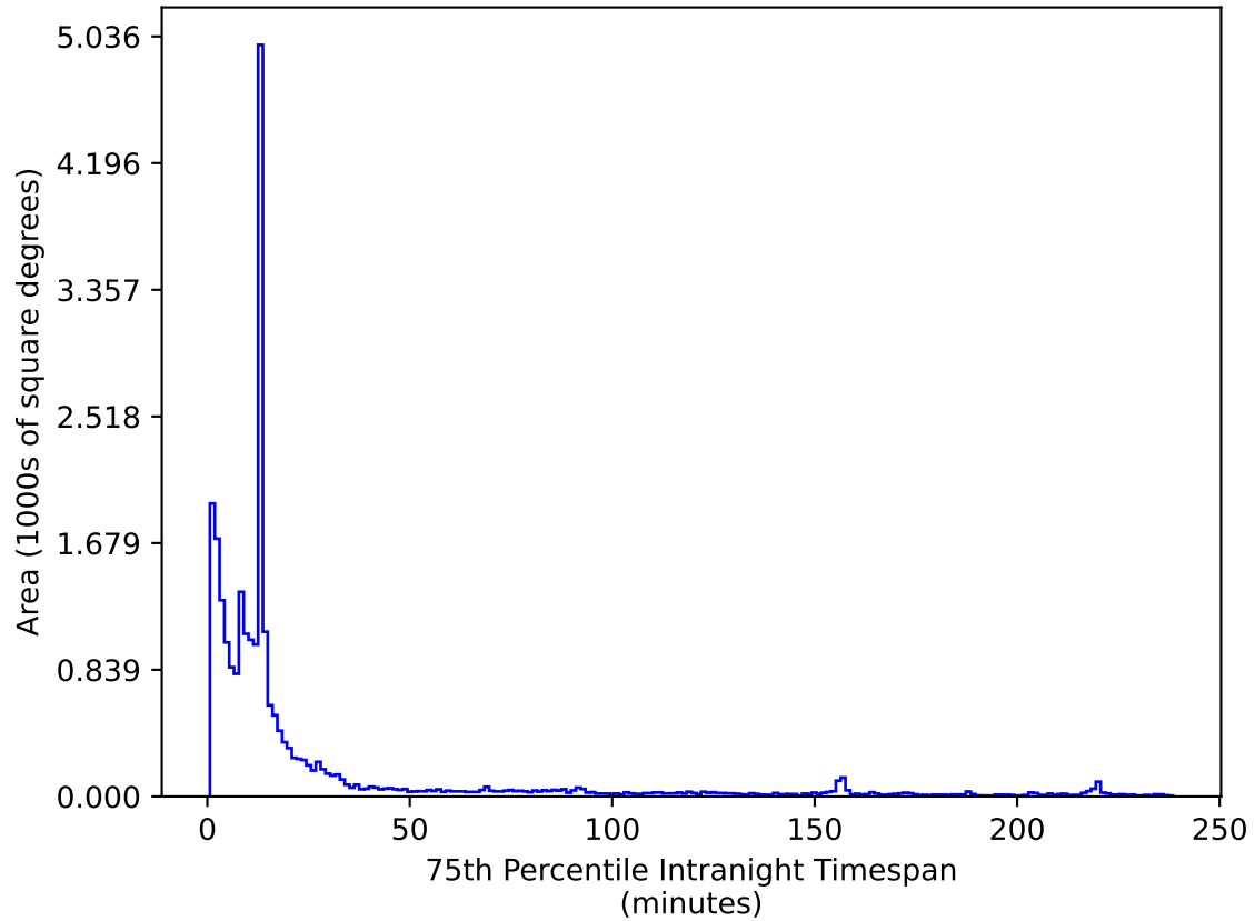
ddf_acor_sf20_lsf0_lsr0_v3.4_10yrs All sky z band: 75th Percentile Intranight Timespan
