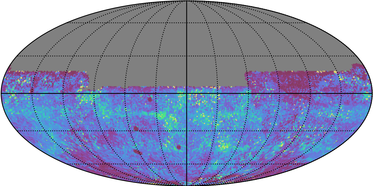
ddf_acor_sf20_lsf0_lsr0_v3.4_10yrs All sky y band: 75th Percentile Intranight Timespan
