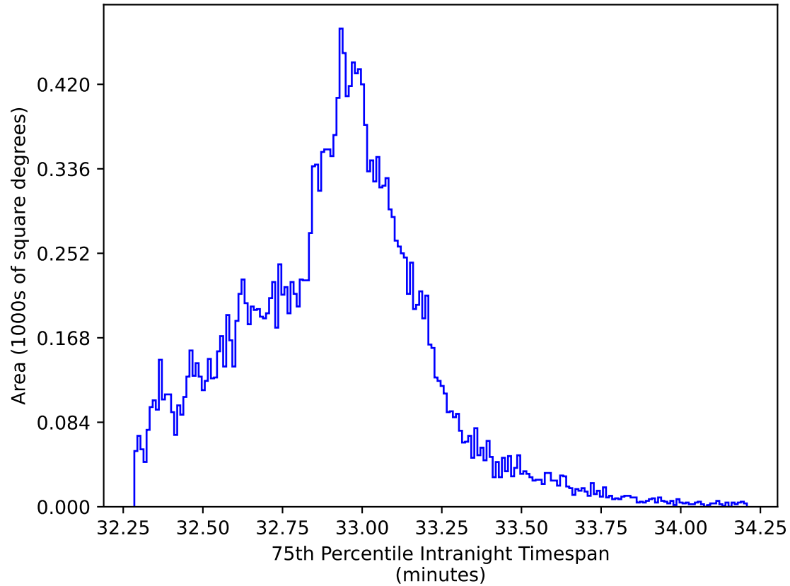
ddf_acor_sf20_ls0_lsr0_v3.4_10yrs All sky y band: 75th Percentile Intranight Timespan
