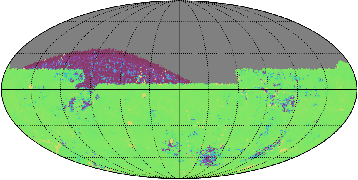
ddf_acor_sf20_lsf0_lsr0_v3.4_10yrs All sky ug bands: 75th Percentile Intranight Timespan
