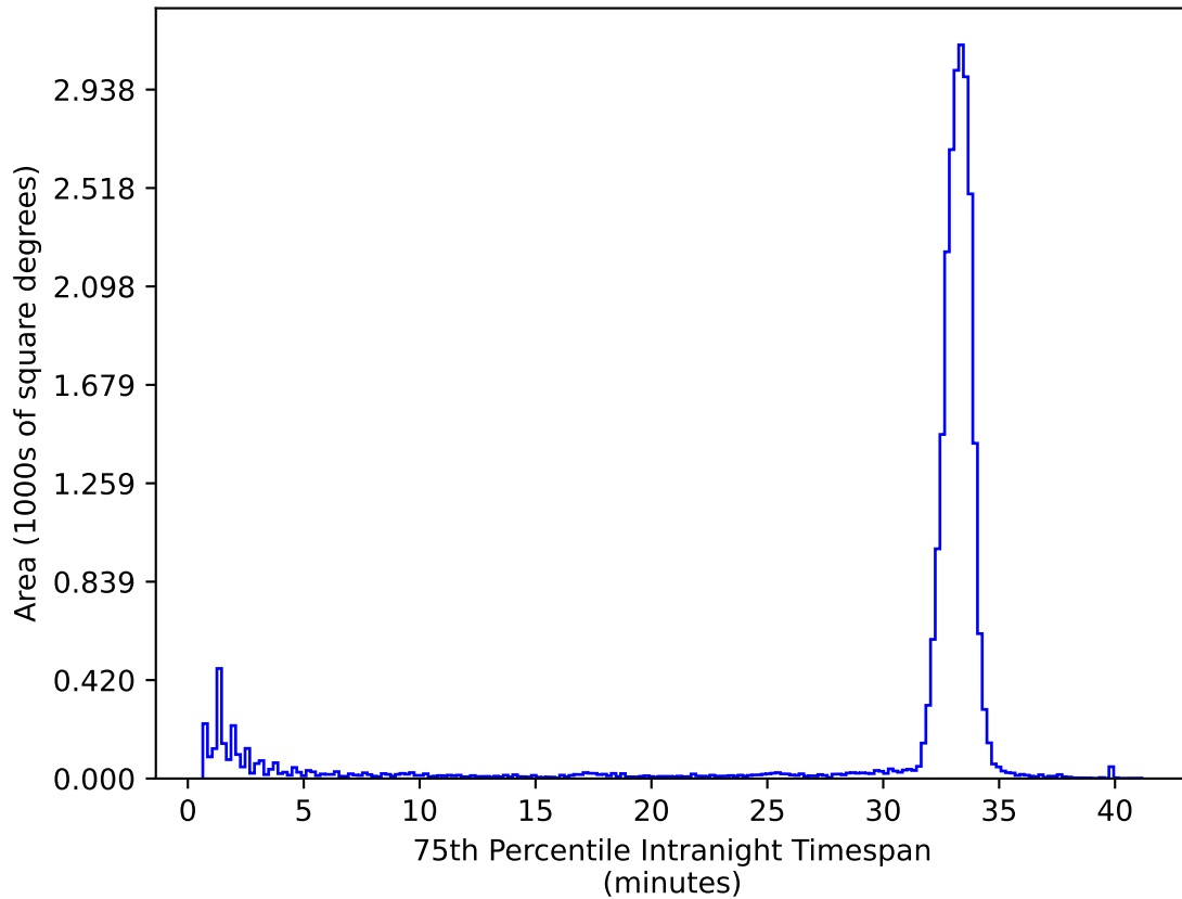
ddf_acor_sf20_lsf0_lsr0_v3.4_10yrs All sky ug bands: 75th Percentile Intranight Timespan
