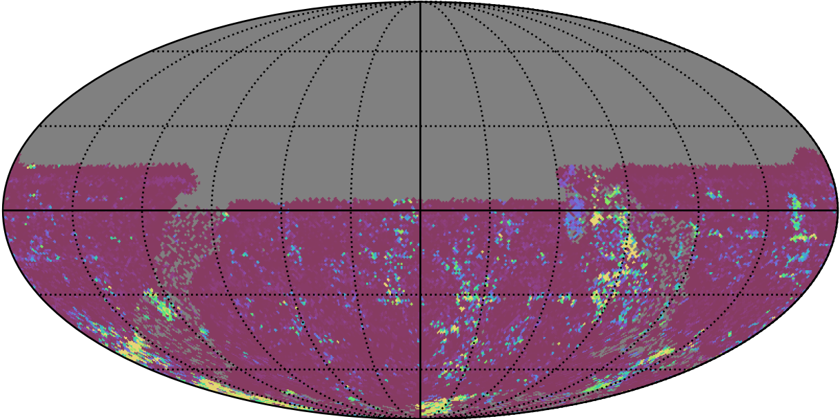
ddf_acor_sf20_lsf0_lsr0_v3.4_10yrs All sky u band: 75th Percentile Intranight Timespan
