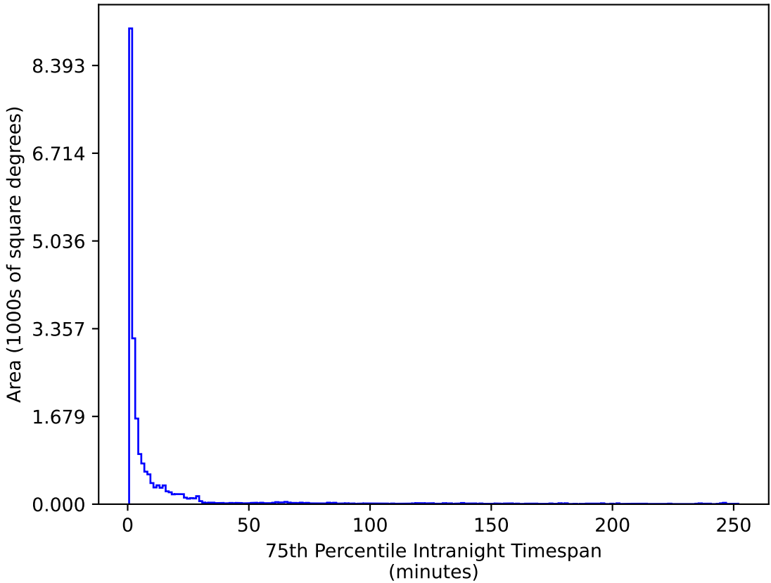
ddf_acor_sf20_lsr0_lsr0_v3.4_10yrs All sky u band: 75th Percentile Intranight Timespan
