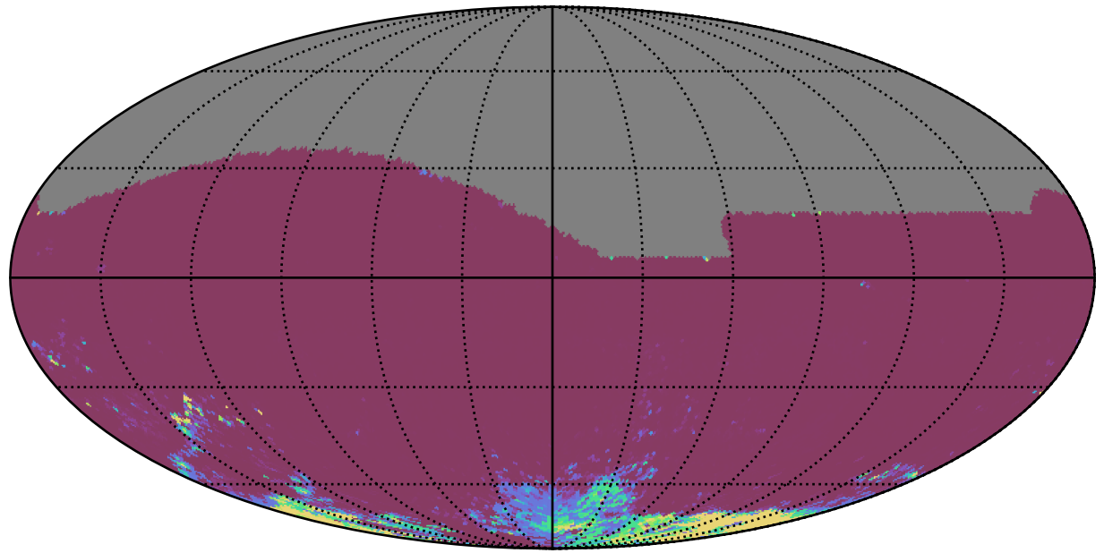
ddf_acor_sf20_lsf0_lsr0_v3.4_10yrs All sky ri bands: 75th Percentile Intranight Timespan
