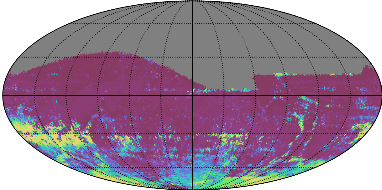
ddf_acor_sf20_lsf0_lsr0_v3.4_10yrs All sky r band: 75th Percentile Intranight Timespan
