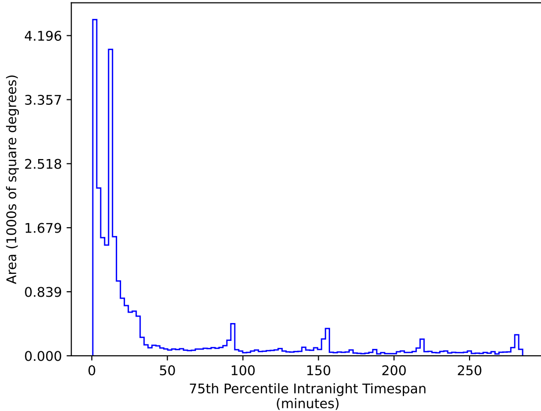
ddf_acor_sf20_ls0_lsr0_v3.4_10yrs All sky r band: 75th Percentile Intranight Timespan
