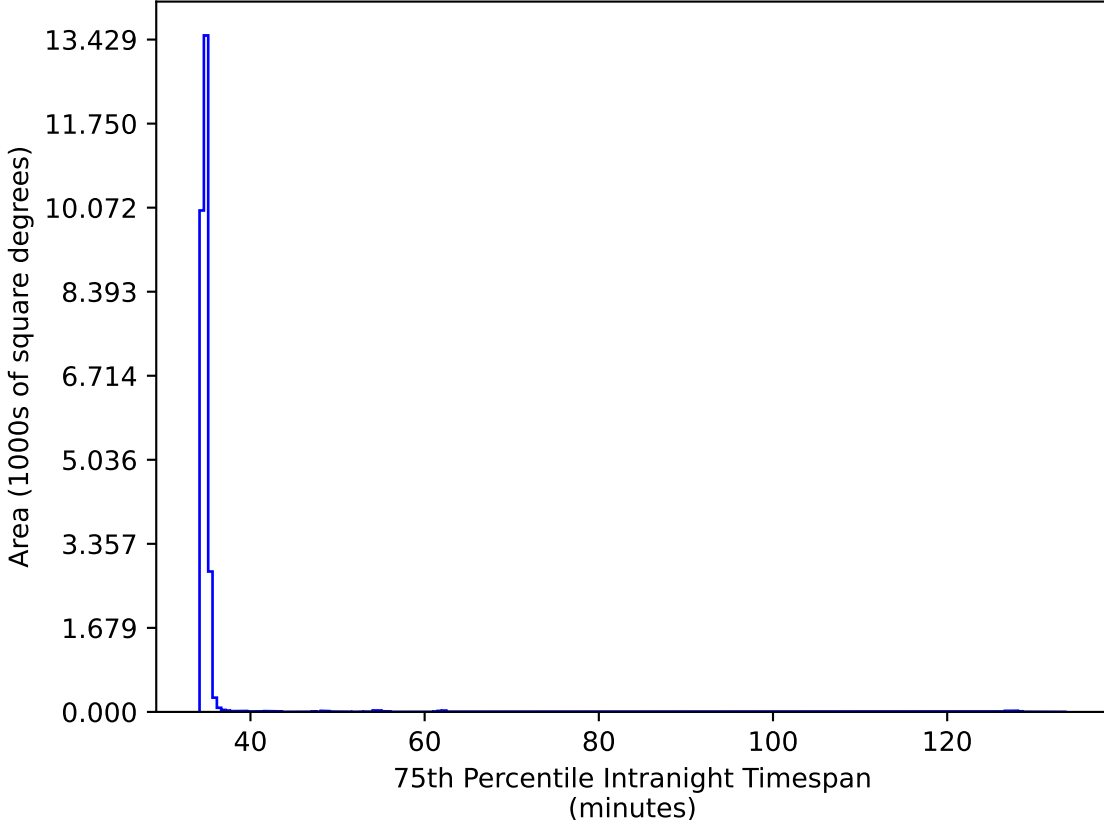
ddf_acor_sf20_lsf0_lsr0_v3.4_10yrs All sky iz bands: 75th Percentile Intranight Timespan
