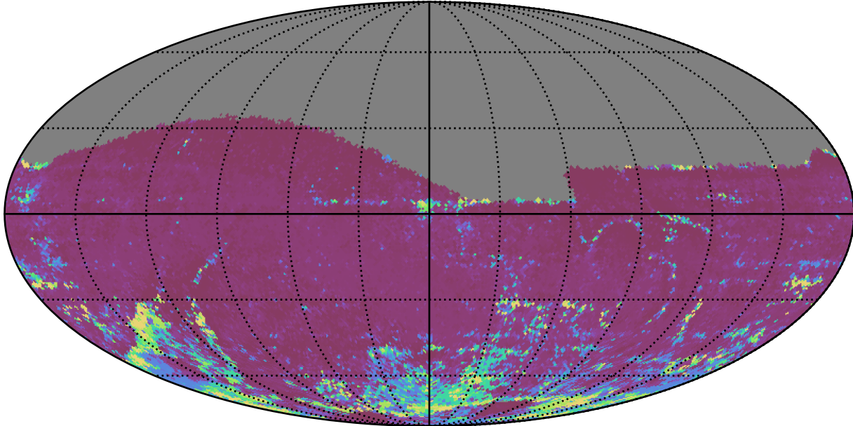
ddf_acor_sf20_lsf0_lsr0_v3.4_10yrs All sky i band: 75th Percentile Intranight Timespan
