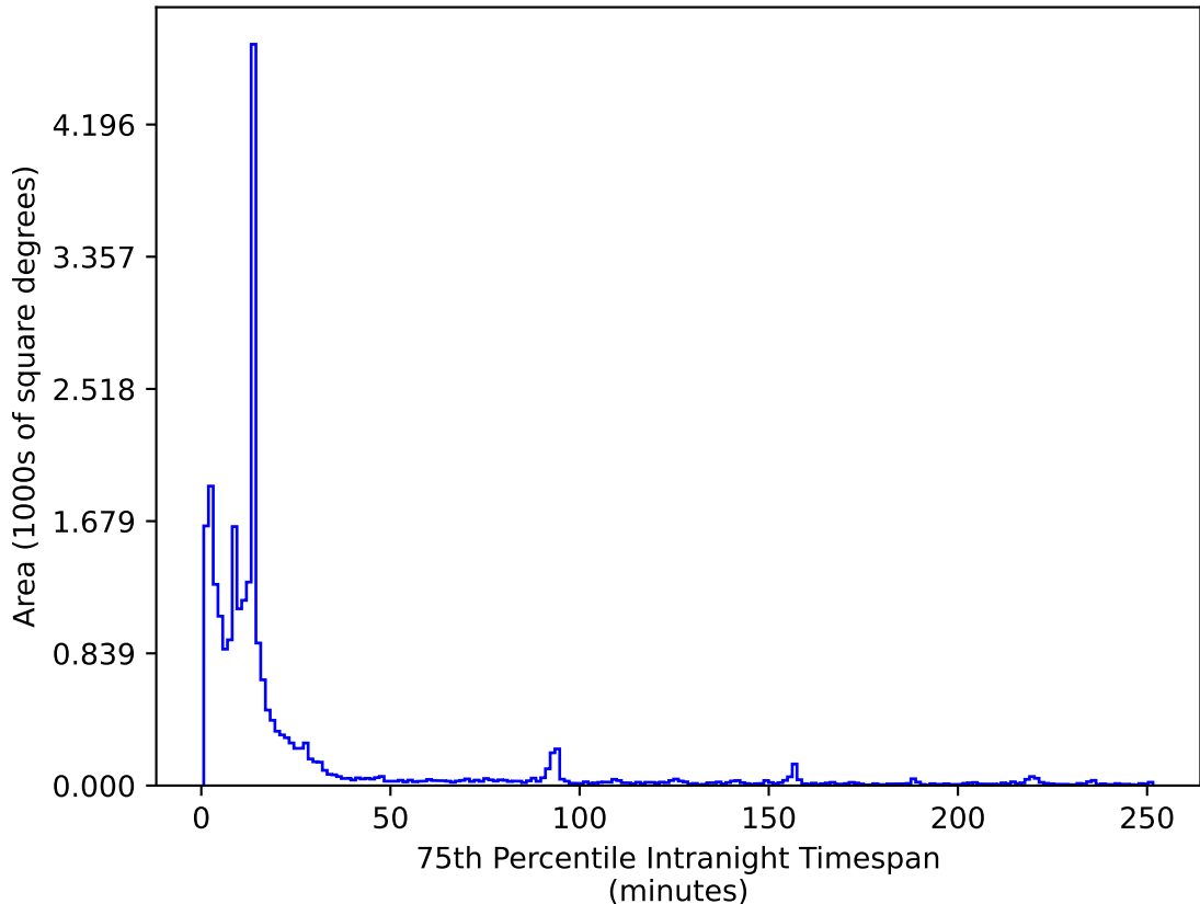
ddf_acor_sf20_lsf0_lsr0_v3.4_10yrs All sky i band: 75th Percentile Intranight Timespan
