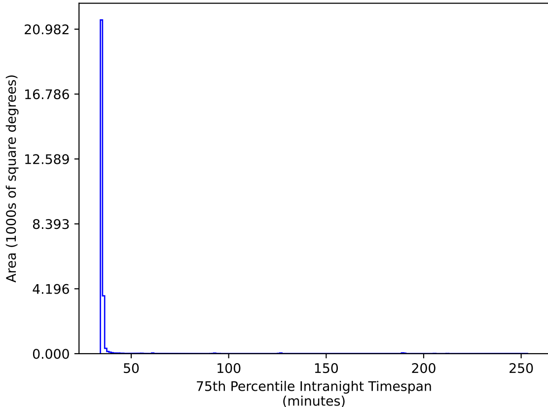
ddf_acor_sf20_lsf0_lsr0_v3.4_10yrs All sky gr bands: 75th Percentile Intranight Timespan
