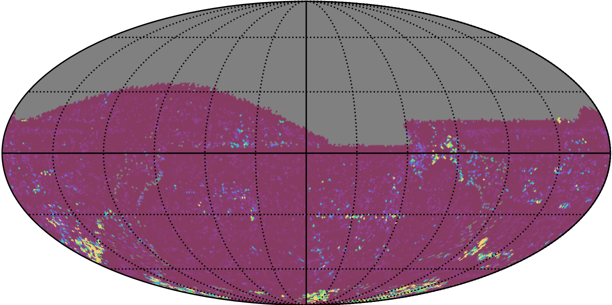
ddf_acor_sf20_lsf0_lsr0_v3.4_10yrs All sky g band: 75th Percentile Intranight Timespan
