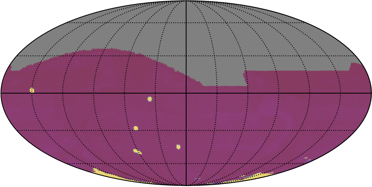
ddf_acor_sf20_lsf0_lsr0_v3.4_10yrs All sky all bands: 75th Percentile Intranight Timespan
