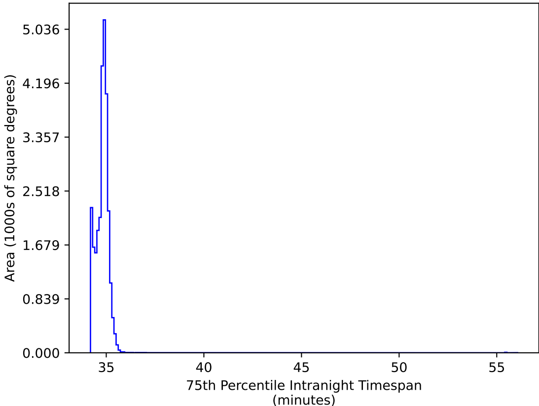
ddf_acor_sf20_lsf0_lsr0_v3.4_10yrs All sky all bands: 75th Percentile Intranight Timespan
