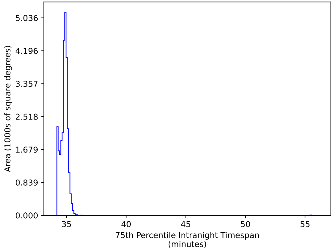
ddf_acor_sf20_lsf0_lsr0_v3.4_10yrs All sky: 75th Percentile Intranight Timespan
