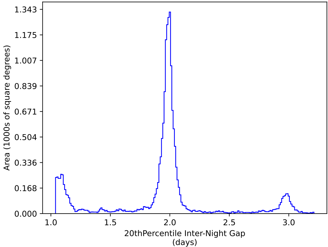
ddf_acor_sf20_lsf0_lsr0_v3.4_10yrs WFD y band: 20thPercentile Inter-Night Gap
