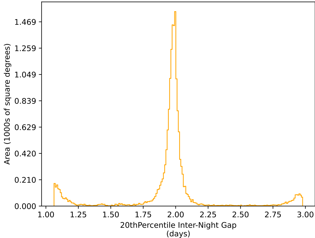
ddf_acor_sf20_lsf0_lsr0_v3.4_10yrs WFD r band: 20thPercentile Inter-Night Gap
