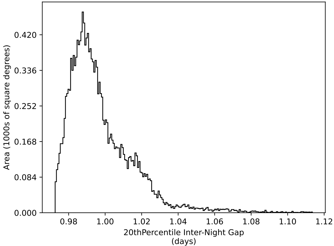
ddf_acor_sf20_ls0_lsr0_v3.4_10yrs WFD all bands: 20thPercentile Inter-Night Gap
