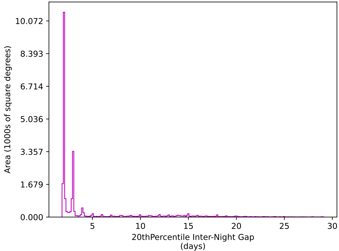
ddf_acor_sf20_lsf0_lsr0_v3.4_10yrs All sky z band: 20thPercentile Inter-Night Gap
