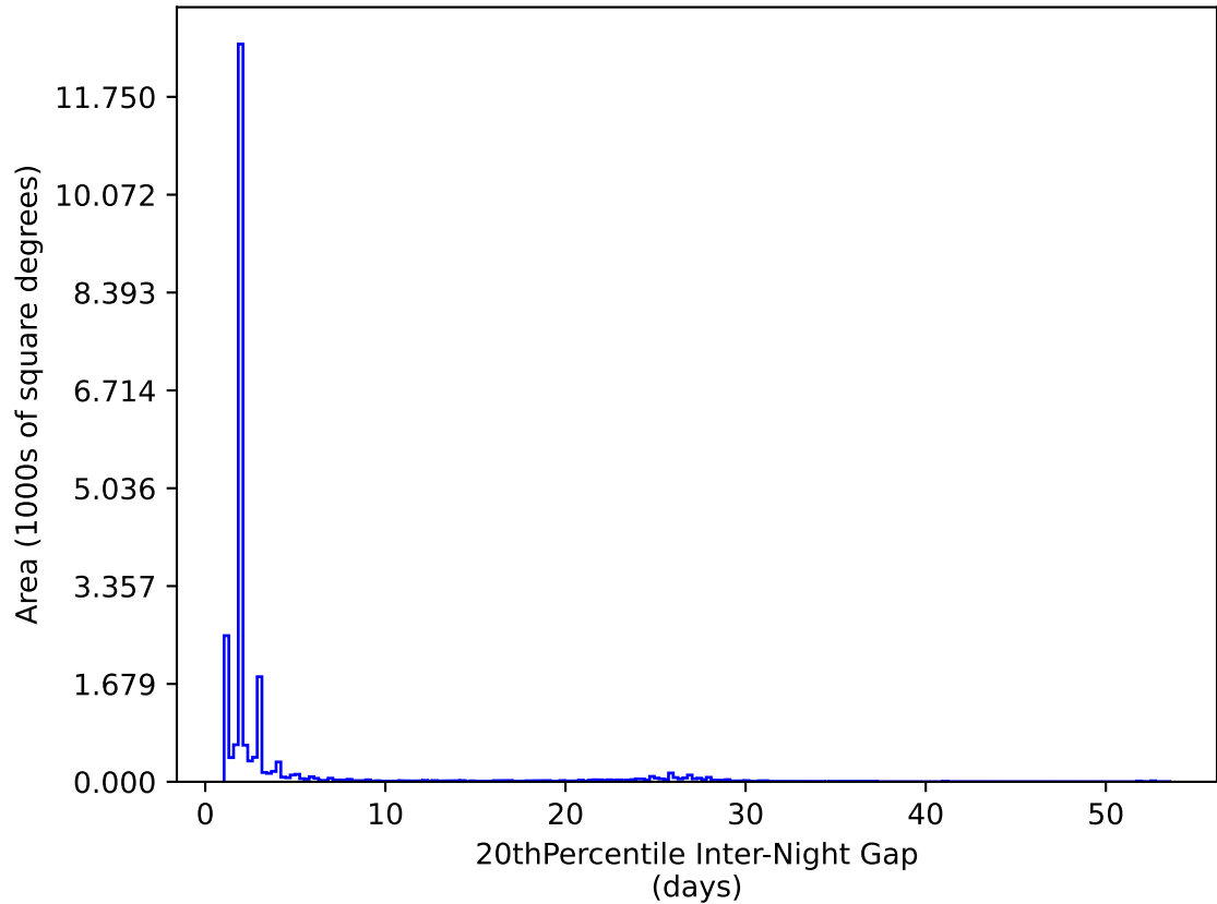
ddf_acor_sf20_lsf0_lsr0_v3.4_10yrs All sky y band: 20thPercentile Inter-Night Gap
