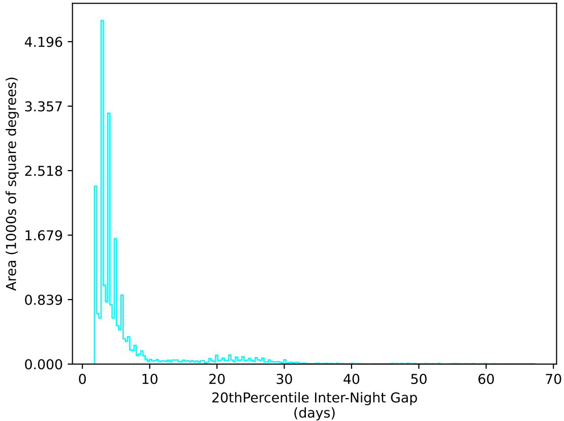
ddf_acor_sf20_lsf0_lsr0_v3.4_10yrs All sky u band: 20thPercentile Inter-Night Gap
