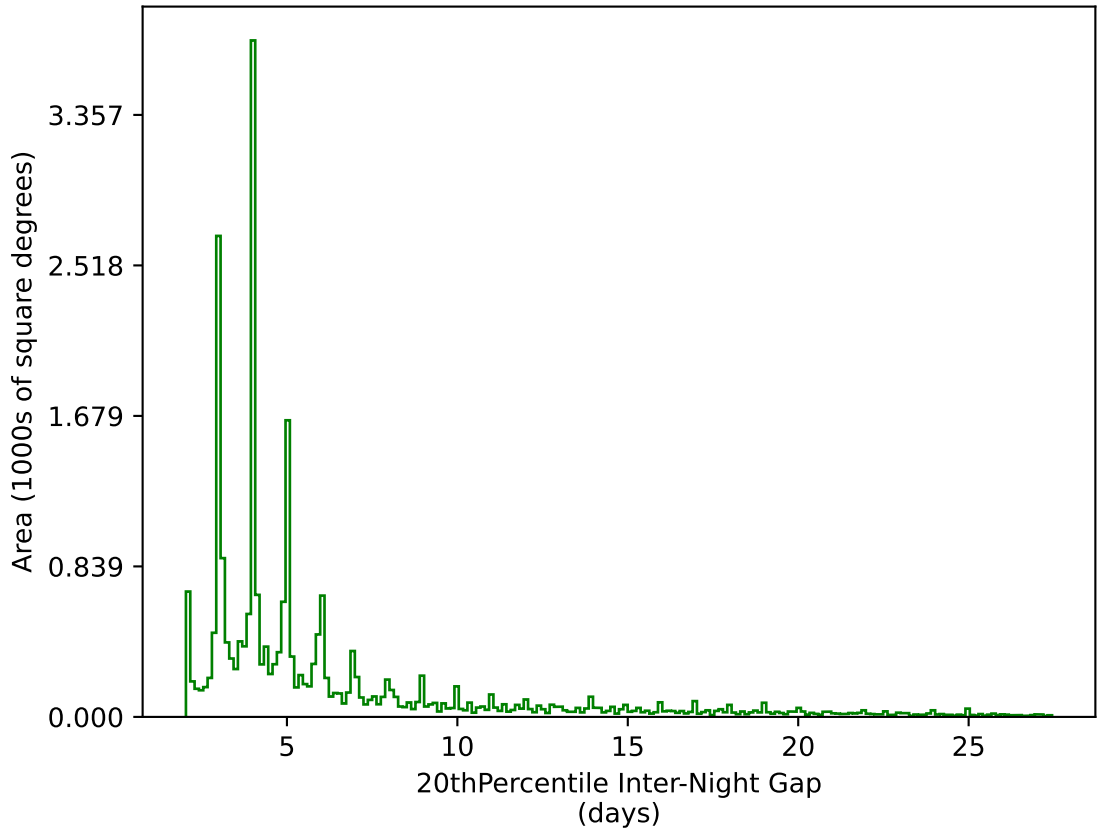
ddf_acor_sf20_ls0_lsr0_v3.4_10yrs All sky g band: 20thPercentile Inter-Night Gap
