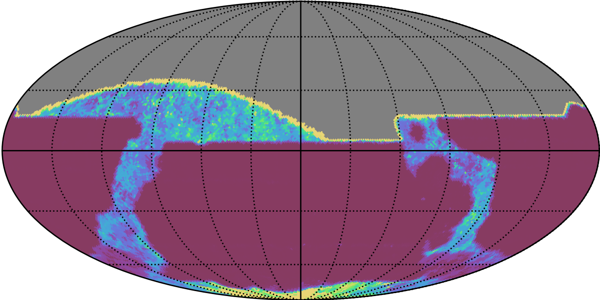
ddf_acor_sf20_lsf0_lsr0_v3.4_10yrs All sky all bands: 20thPercentile Inter-Night Gap
