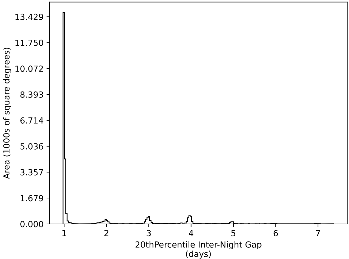
ddf_acor_sf20_lsf0_lsr0_v3.4_10yrs All sky all bands: 20thPercentile Inter-Night Gap
