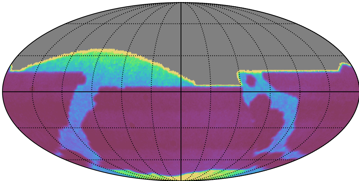
ddf_acor_sf20_lsf0_lsr0_v3.4_10yrs : properMotion
