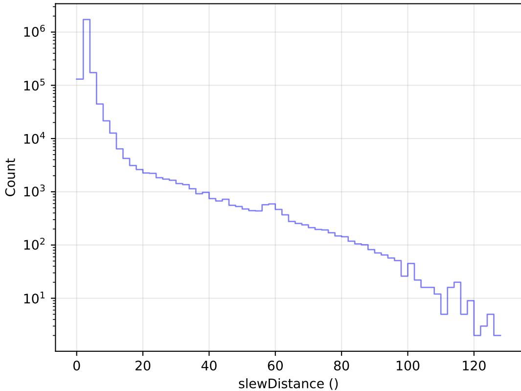
ddf_acor_sf20_lsf0_lsr0_v3.4_10yrs All visits: Slew Distance Histogram
