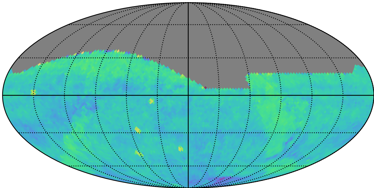
ddf_acor_sf20_lsf0_lsr0_v3.4_10yrs (g or r or i): PairFraction
