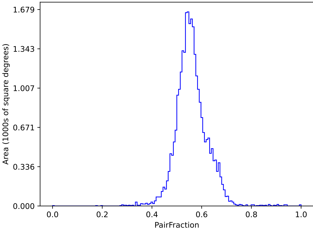
ddf_acor_sf20_lsf0_lsr0_v3.4_10yrs (g or r or i): PairFraction
