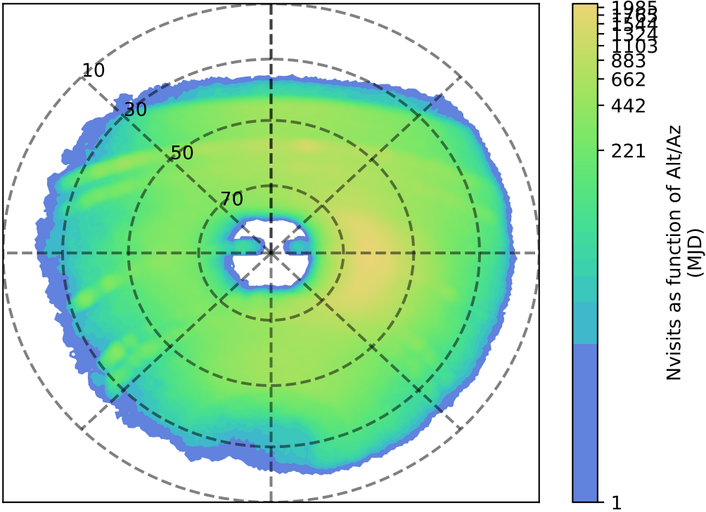
ddf_acor_sf20_lsf0_lsr0_v3.4_10yrs y: Nvisits as function of Alt/Az
