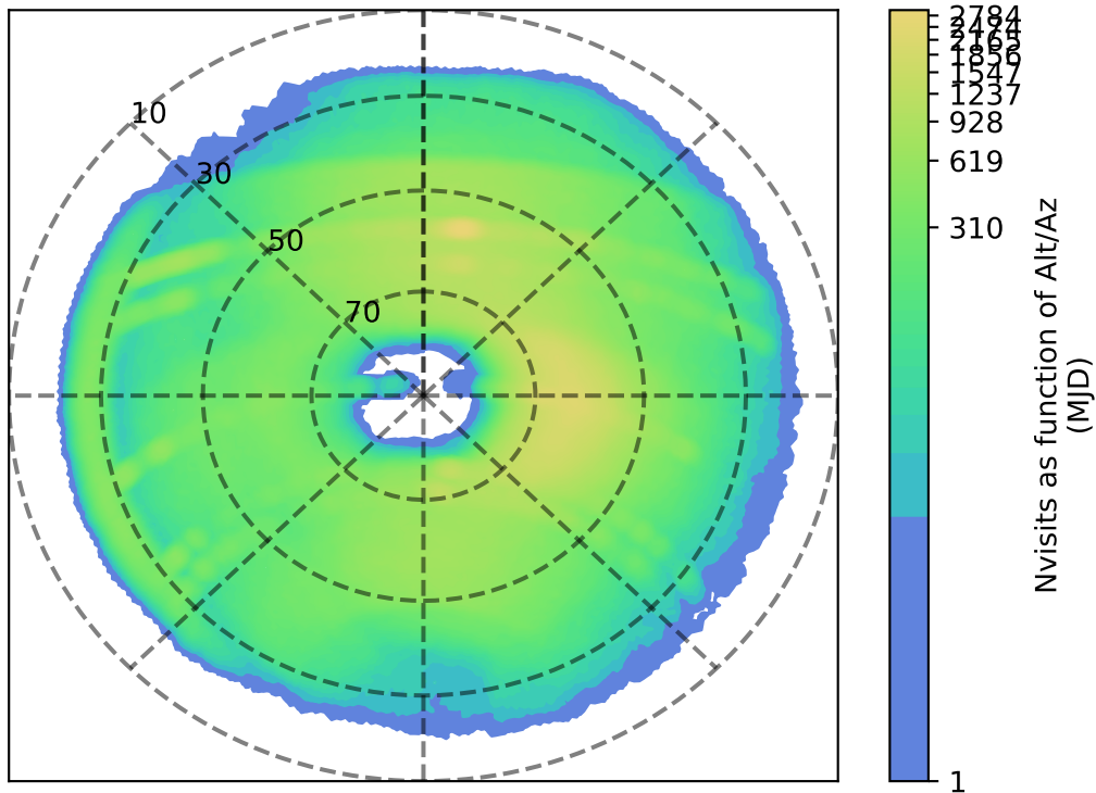
ddf_acor_sf20_lsf0_lsr0_v3.4_10yrs r: Nvisits as function of Alt/Az
