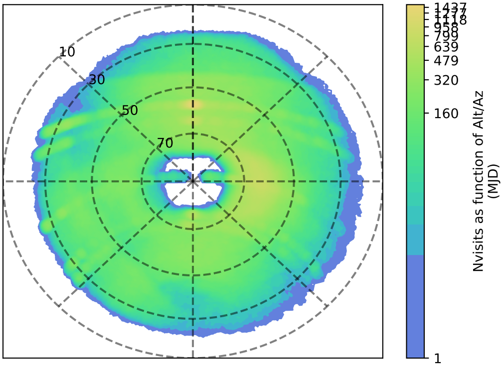
ddf_acor_sf20_lsf0_lsr0_v3.4_10yrs g: Nvisits as function of Alt/Az
