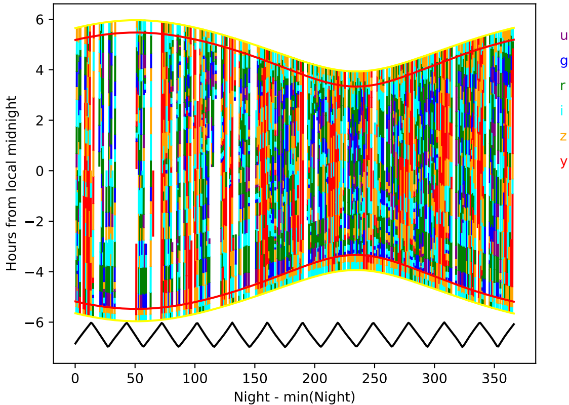
ddf_acor_sf20_lsf0_lsr0_v3.4_10yrs year 8-9: Hourglass
