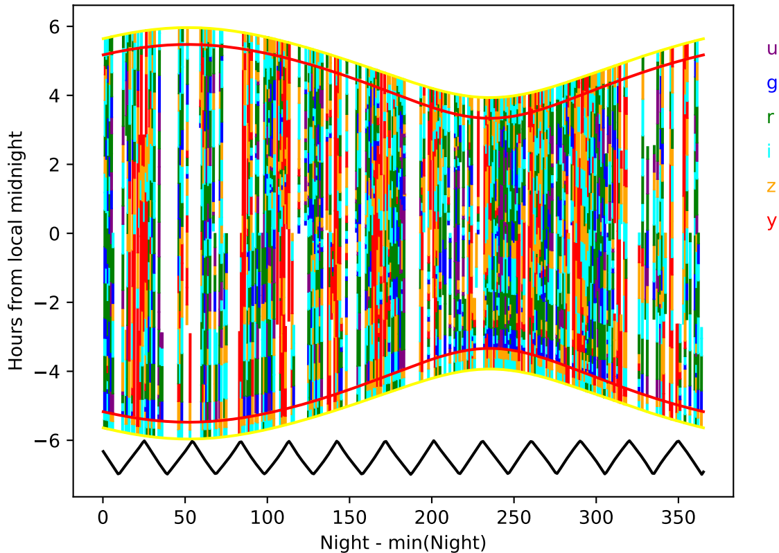
ddf_acor_sf20_lsf0_lsr0_v3.4_10yrs year 7-8: Hourglass
