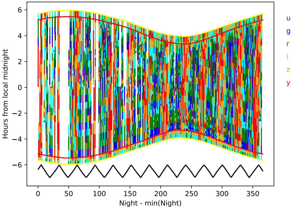
ddf_acor_sf20_lsf0_lsr0_v3.4_10yrs year 6-7: Hourglass
